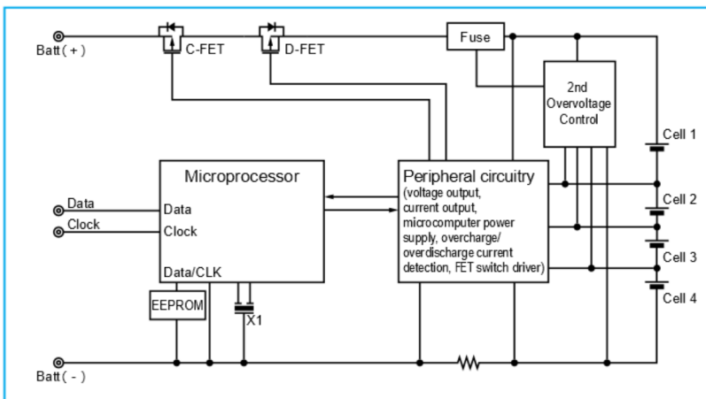
(fig.39) Peripheral circuitry (voltage output, current output, microprocessor power supply, overcharge/overdischarge current detection, FET switch drivers)
